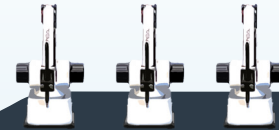
SketchBots
