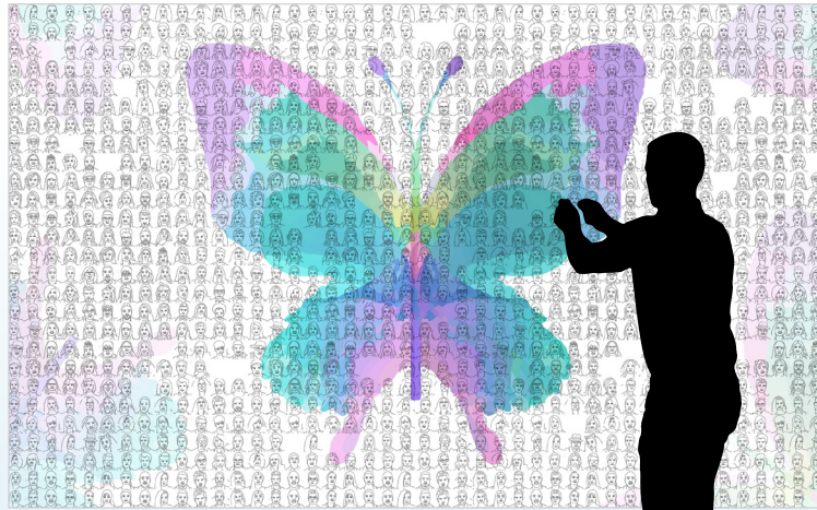
SketchBot Mosaic
